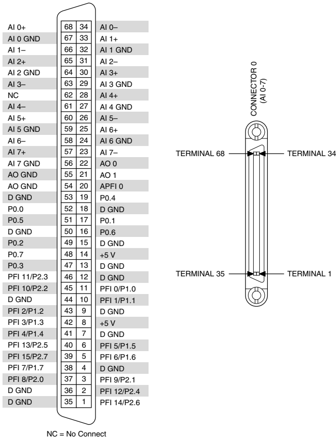
Figure 6. NI PXle-6376 Pinout
